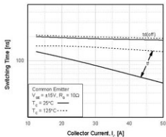
Figure 12. Turn-Off Characteristics vs. Collector Current
