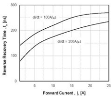
Figure 21. Reverse Recovery Time
