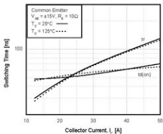
Figure 11. Turn-On Characteristics vs. Collector Current
