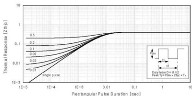
Figure 17. Transient Thermal Impedance of IGBT
