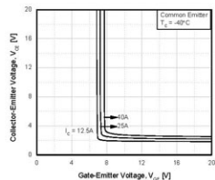
Figure 6. Saturation Voltage vs. V_{GE}
