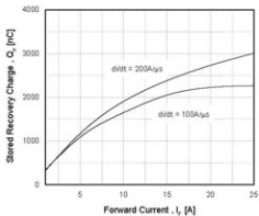
Figure 20. Stored Charge
