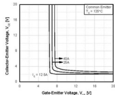
Figure 6. Saturation Voltage vs. V_{GE}
