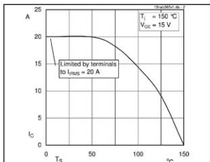
Fig. 2 Typ. rated current vs. temperature
