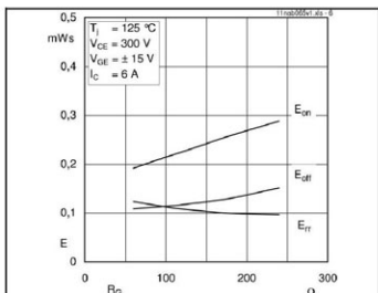
Fig. 6 Typ. Turn-on / off energy = f(R_c)
