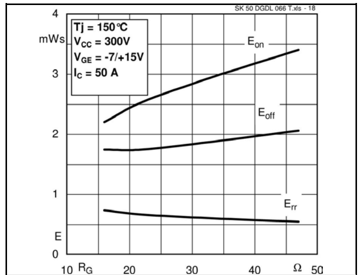
Fig.18 Turn-on/-off energy=f(Rg)
