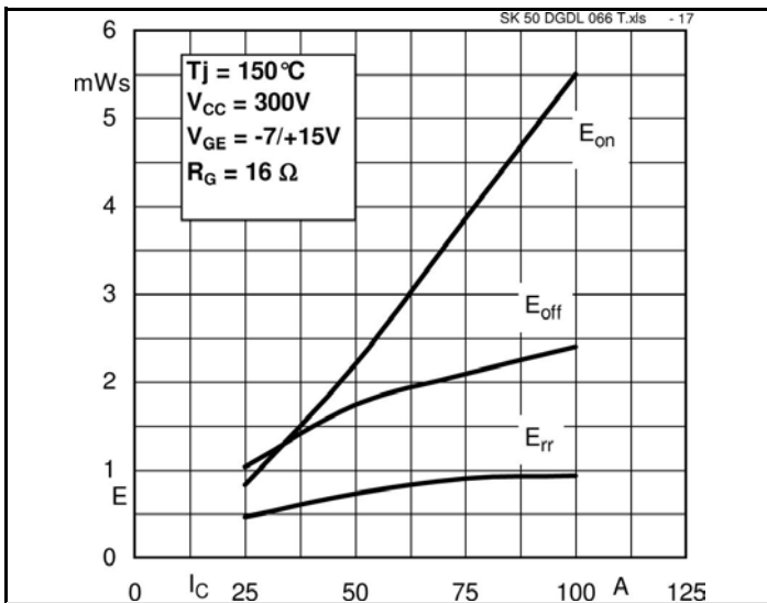
Fig.17 Turn-on/-off energy=f(Ic)
