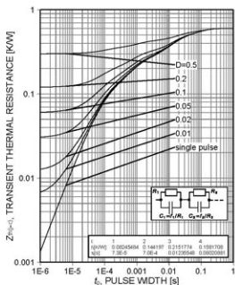
Figure 18. IGBT transient thermal resistance ( D=t_i/T )
