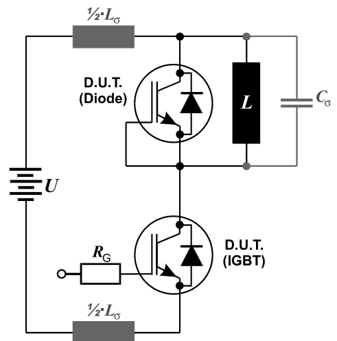
Figure E. Dynamic test circuit Leakage inductance L_S = 180\text{nH} and Stray capacity C_S = 39\text{pF} .
