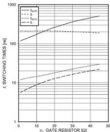
Figure 10. Typical switching times as a function of gate resistor (inductive load, T_j=175^{\circ}\text{C} , V_{CE}=400\text{V} , V_{GE}=150\text{V} , I_C=15\text{A} , Dynamic test circuit in Figure E)
