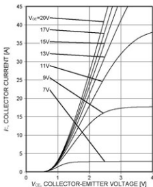
Figure 5. Typical output characteristic ( T_c=25^\circ\text{C} )
