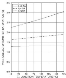
Figure 8. Typical collector-emitter saturation voltage as a function of junction temperature ( V_{CE}=15\text{V} )
