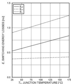
Figure 15. Typical switching energy losses as a function of junction temperature (inductive load, V_{CE}=400\text{V} , V_{GE}=15/0\text{V} , I_C=15\text{A} , r_{\theta jc}=15\Omega , Dynamic test circuit in Figure E)
