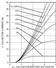
Figure 6. Typical output characteristic ( T_c=175^\circ\text{C} )
