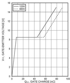
Figure 17. Typical gate charge ( I_C=15A )
