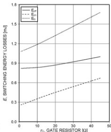
Figure 14. Typical switching energy losses as a function of gate resistor (inductive load, T_j=175^{\circ}\text{C} , V_{CE}=400\text{V} , V_{GE}=15/0\text{V} , I_C=15\text{A} , Dynamic test circuit in Figure E)
