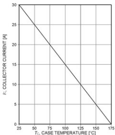
Figure 4. Collector current as a function of case temperature ( V_{CE} \geq 15\text{V} , T_J \leq 175^\circ\text{C} )
