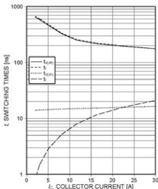
Figure 9. Typical switching times as a function of collector current (inductive load, T_j=175^{\circ}\text{C} , V_{CE}=400\text{V} , V_{GE}=150\text{V} , r_{GS}=15\Omega , Dynamic test circuit in Figure E)
