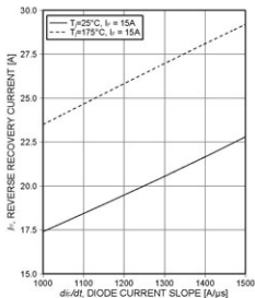
Figure 25. Typical reverse recovery current as a function of diode current slope ( V_{rr}=400V )
