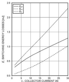
Figure 13. Typical switching energy losses as a function of collector current (inductive load, T_j=175^{\circ}\text{C} , V_{CE}=400\text{V} , V_{GE}=15/0\text{V} , I_C=15\text{A} , r_{\theta jc}=15\Omega , Dynamic test circuit in Figure E)
