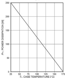
Figure 3. Power dissipation as a function of case temperature ( T_C \leq 175^\circ\text{C} )
