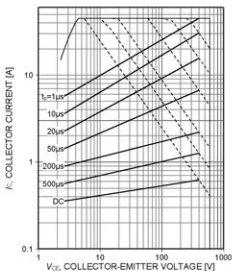
Figure 2. Forward bias safe operating area ( D = 0 , T_C = 25^\circ\text{C} , T_J \leq 175^\circ\text{C} , V_{CE} = 15\text{V} )
