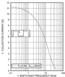
Figure 1. Collector current as a function of switching frequency ( T_C \leq 175^\circ\text{C} , T_J = 55^\circ\text{C} , D = 0.5 , V_{CE} = 400\text{V} , V_{CE} = 150\text{V} , f_{\text{sw}} = 15\text{kHz} , PCB mounting with thermal vias and heatsink, see Appnote: www.infineon.com/igbt )
