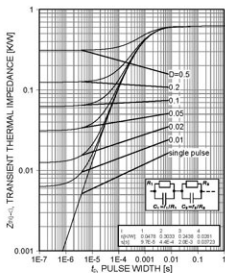
Figure 21. IGBT transient thermal impedance 1) ( D=t_p/T )
