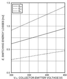
Figure 16. Typical switching energy losses as a function of collector emitter voltage (inductive load, T_j=175^{\circ}\text{C} , V_{GE}=15/0\text{V} , I_C=15\text{A} , r_{\theta jc}=15\Omega , Dynamic test circuit in Figure E)
