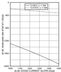
Figure 26. Typical diode peak rate of fall of reverse recovery current as a function of diode current slope ( V_{rr}=400V )
