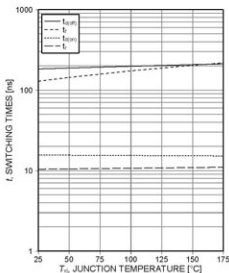
Figure 11. Typical switching times as a function of junction temperature (inductive load, V_{CE}=400\text{V} , V_{GE}=150\text{V} , I_C=15\text{A} , r_{GS}=15\Omega , Dynamic test circuit in Figure E)
