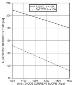
Figure 23. Typical reverse recovery time as a function of diode current slope ( V_c=400V )
