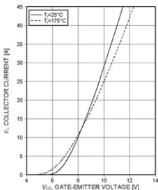
Figure 7. Typical transfer characteristic ( V_{CE}=10\text{V} )
