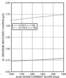
Figure 24. Typical reverse recovery charge as a function of diode current slope ( V_c=400V )
