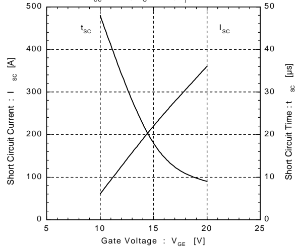
Typical Short Circuit Capability V CC =400V, R G =8.2Ω, T J =125°C
