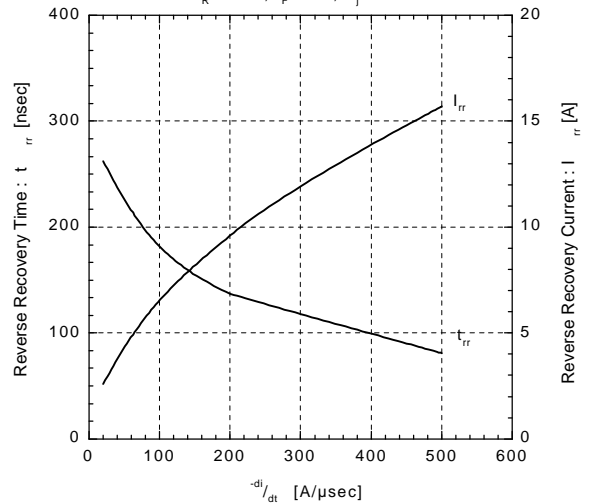
Reverse Recovery Characteristics vs. -di/dt V R =200V, I F =30A, T J =125°C
