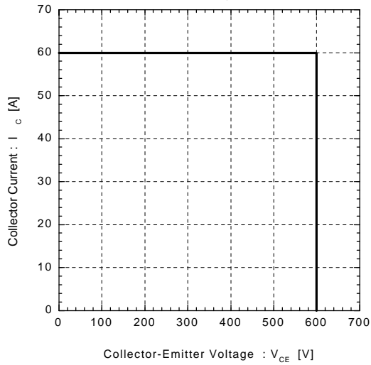
Reverse Biased Safe Operating Area +V GE =15V, -V GE ≤15V, T J ≤125°C, R G ≥8.2Ω
