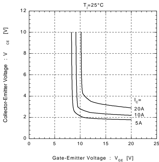
Collector-Emittter Voltage vs. Gate-Emittter Voltage
