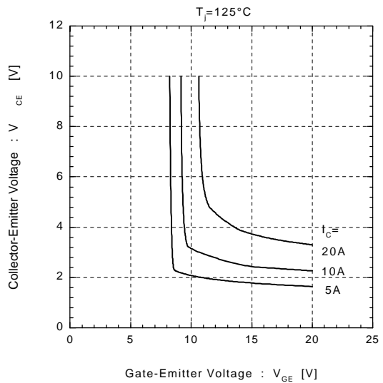
Collector-Emittter Voltage vs. Gate-Emittter Voltage
