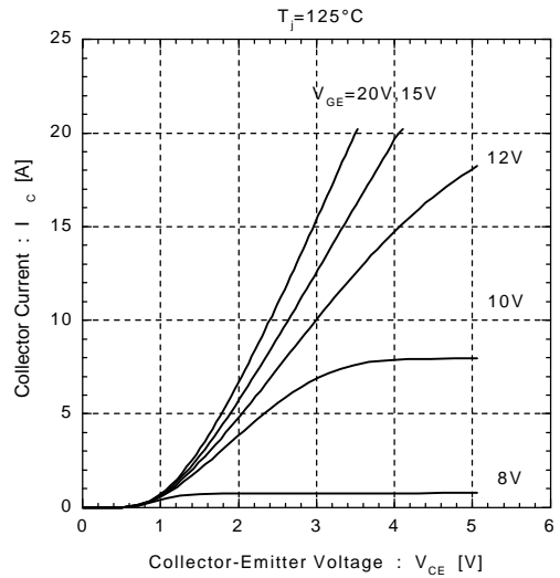
Collector Current vs. Collector-Emittter Voltage
